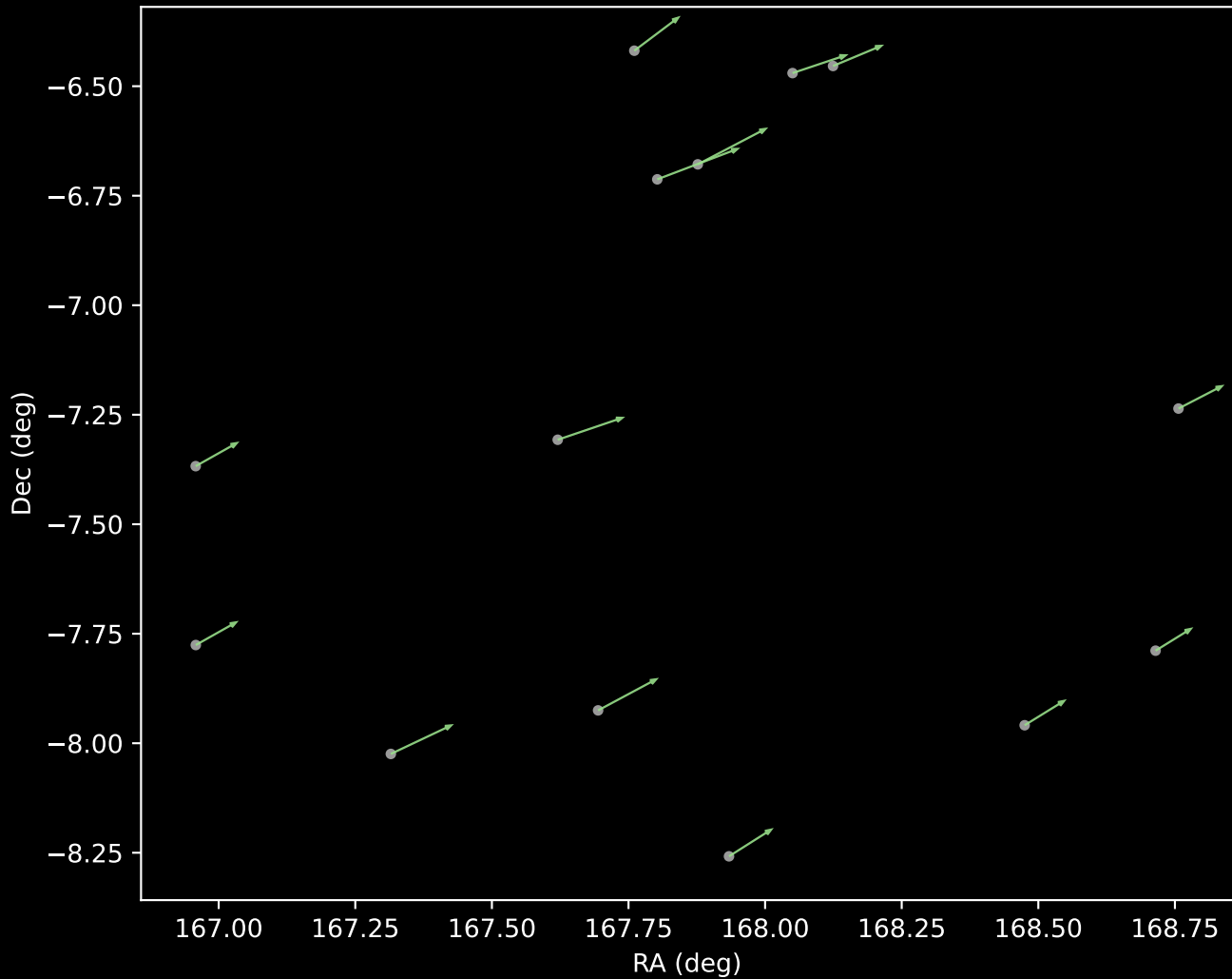
GALAH DR4 Cluster 5 Proper Motion Vectors (n=14)
