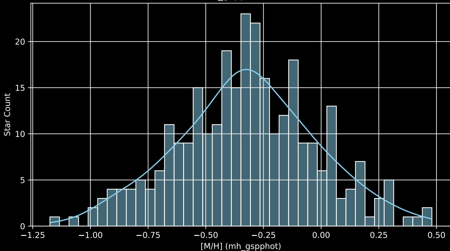
GALAH DR4 Field: [617] [M/H] (mh_gspphot) (n= 298)
