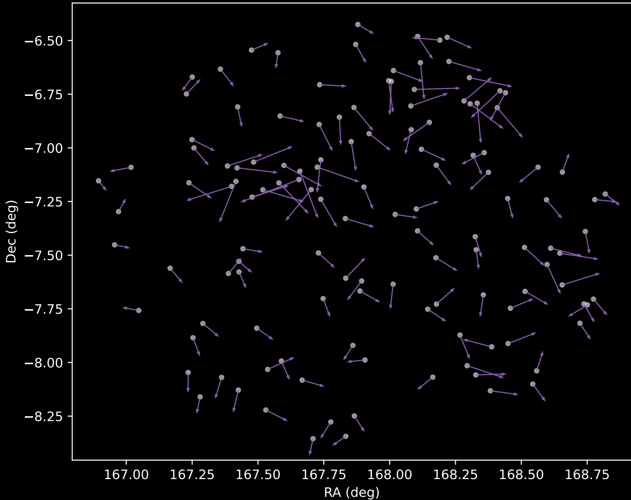
GALAH DR4 Cluster 8 Proper Motion Vectors (n=128)
