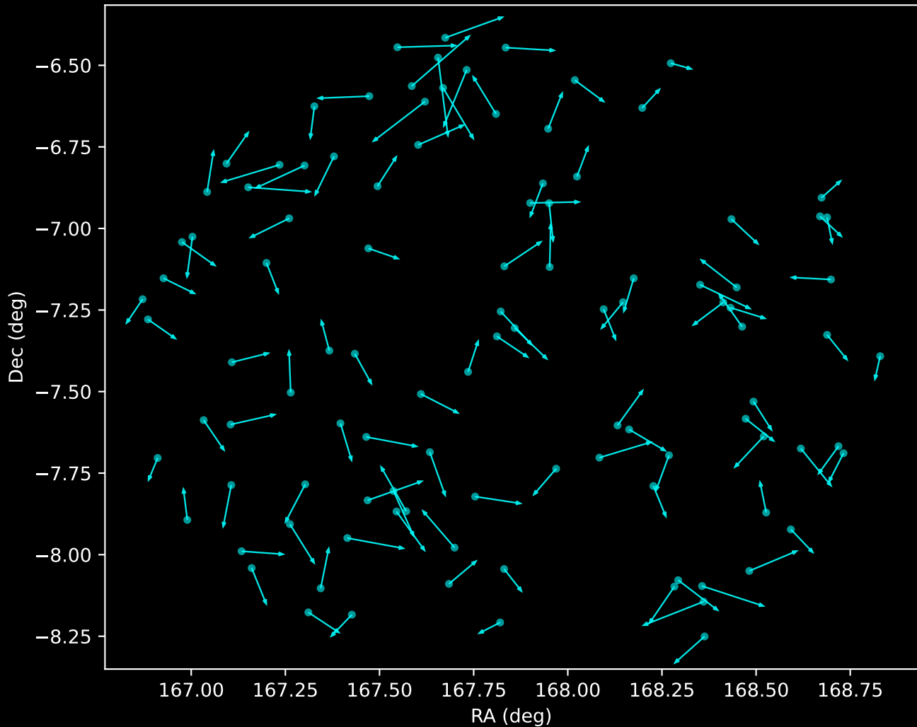
GALAH DR4 Noise Stream Proper Motion Vectors (n=106)
