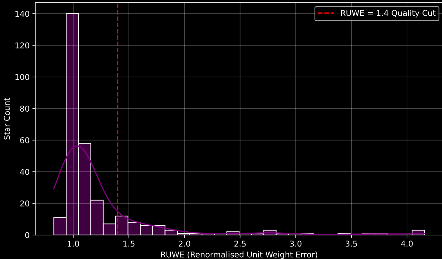
GALAH DR4 Field [617] RUWE Distribution (n= 290)
