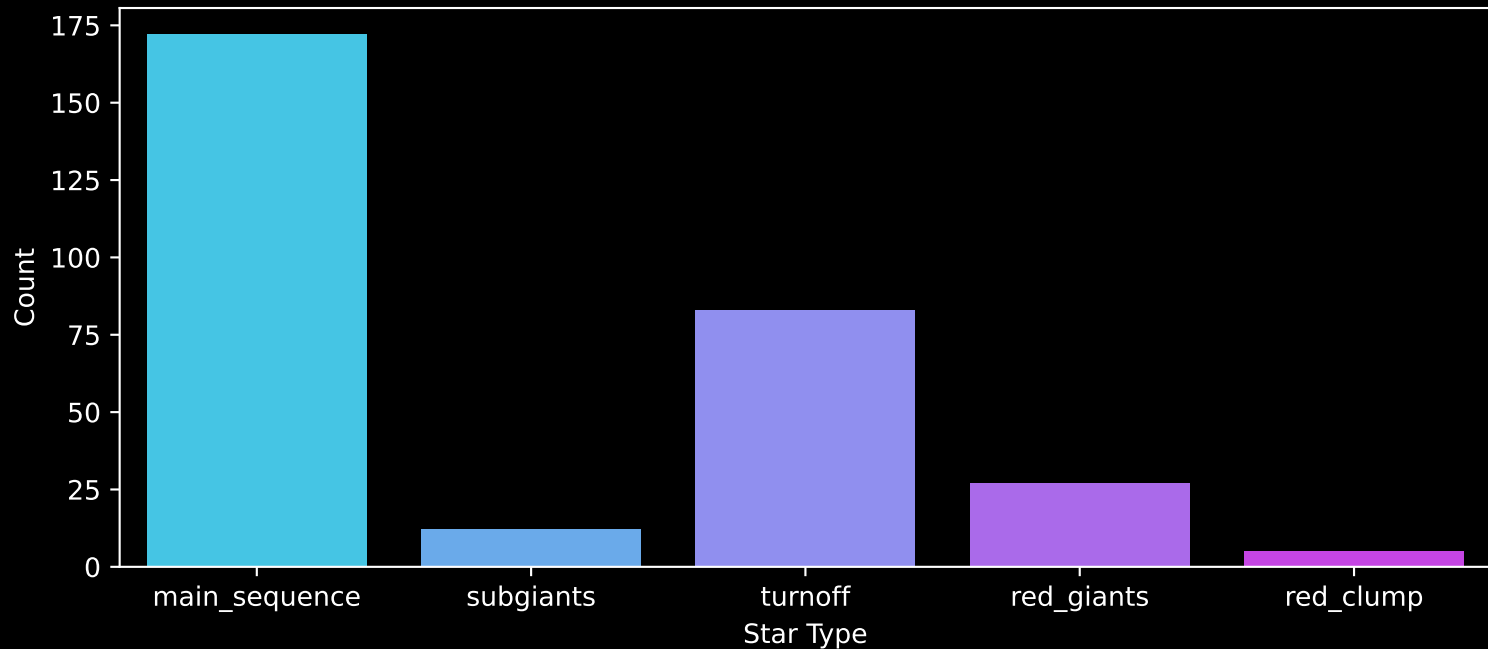
GALAH DR4 Field: [617] Count plot of Star Type
