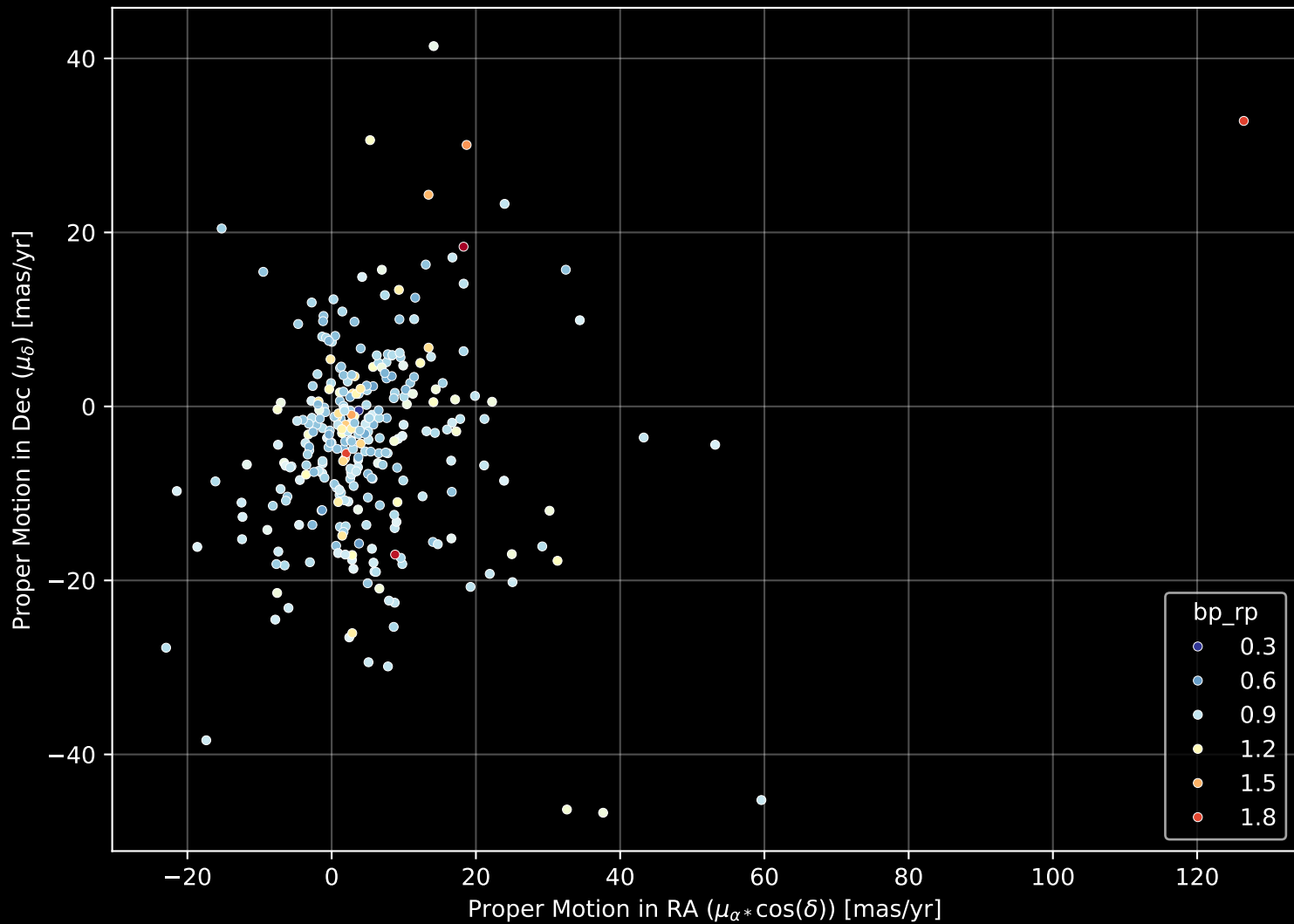
GALAH DR4 Field: [617] Proper Motion Diagram (n= 299)
